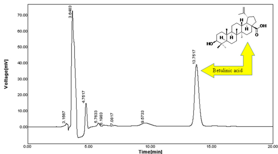
Figure 1: The RP-HPLC profile of betulinic acid as reference compound (conc.100ppm)
