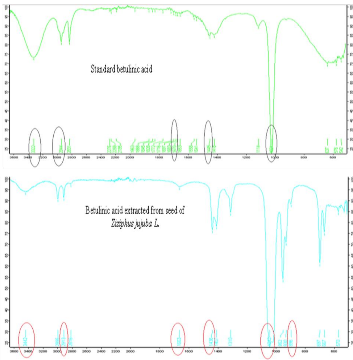
Figure 4: Comparative FT-IR profile of (A) standard betulinic acid shown in green color (B) betulinic acid extracted from seed of mature fruits of Ziziphus jujuba L. shown in blue color. The circles represent similar bond stretches in standard betulinic acid & extracted sample from seed of mature fruits of Ziziphus jujuba L.
